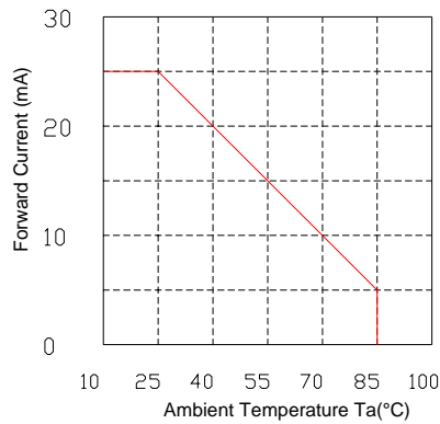
Derating
