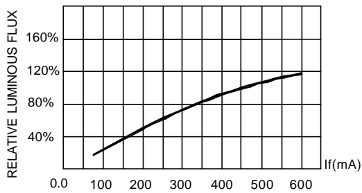
FIG.2 FORWARD CURRENT.
