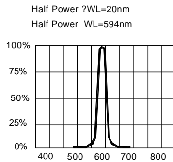
FIG.3 RELATIVE LUMINOUS FLUX VS. WAVELENGTH.
