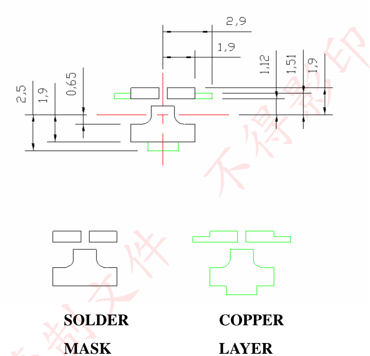
Fig.10 Solder Pad Layout.
